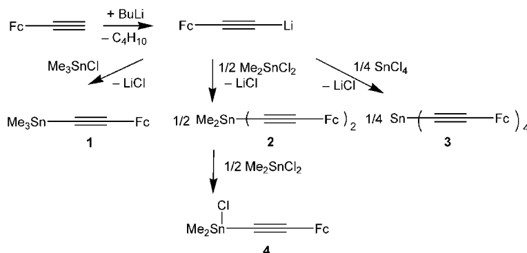
Scheme 2. Synthesis of the ferrocenylethynyltin compounds (Fc = Ferrocenyl).
