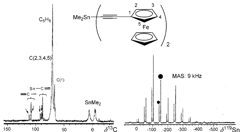
Figure 4. Solid-state VACP [27] MAS 13 C{ 1 H} (100.5 MHz) and 119 Sn{ 1 H} (149.1 MHz) NMR spectra of 2 , showing the presence of two modifications in the crystalline state. The signals for the isotropic \delta_{119\text{Sn}} values are marked by filled circles. The alkynyl 13 C NMR signals for the modification that is not represented by the crystal structure (Figure 3) are marked by arrows.
