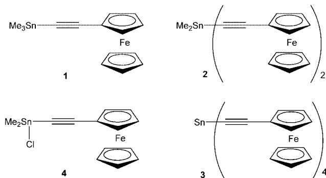
Scheme 1. The ferrocenylethynyltin compounds studied.
