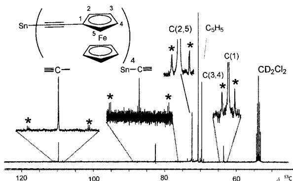
Figure 1. ^{13}\text{C}\{^1\text{H}\} NMR spectrum (100.5 MHz) of tetrakis(ferrocenylethynyl)tin ( 3 ; saturated solution in \text{CD}_2\text{Cl}_2 ) showing the ^{117/119}\text{Sn} satellites (marked by asterisks) for spin-spin coupling across one, two, three, and four bonds.
