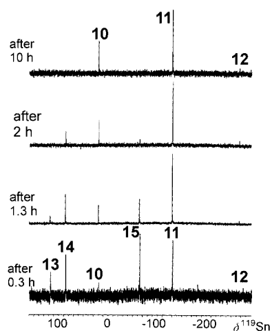
Figure 6. ^{119}\text{Sn}\{^1\text{H}\text{-inverse-gated}\} NMR spectra (149.1 MHz) of the \text{CD}_2\text{Cl}_2 solution from the reaction of tetrakis(ferrocenylethynyl)tin ( 3 ) with an excess of \text{BEt}_3 . ^{119}\text{Sn} NMR signals of the zwitterionic intermediates 13 – 15 are observed in the beginning, and after 10 h at room temperature only ^{119}\text{Sn} NMR signals of the spirotin compounds 10 , 11 and 12 (ratio 45:50:5) are left.
