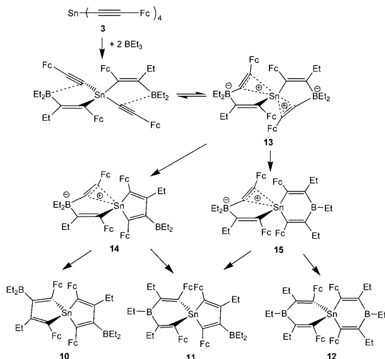
Scheme 5. 1,1-Ethylboration of tetrakis(ferrocenylethynyl)tin ( 3 ).
