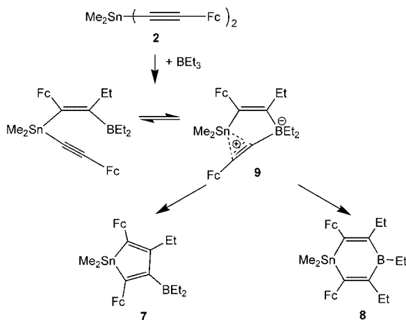
Scheme 4. 1,1-Organoboration of the bis(ferrocenylethynyl)dimethyltin ( 2 ).
