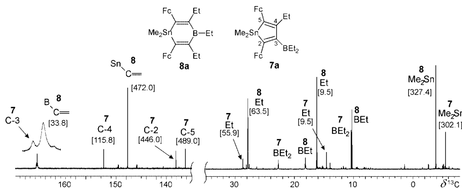
Figure 5. ^{13}\text{C}\{^1\text{H}\} NMR spectrum (100.5 MHz) of the mixture of products 7a and 8a showing the assigned ^{13}\text{C} NMR signals in the ranges expected for the olefinic and the aliphatic carbon atoms. ^{117/119}\text{Sn} satellites are indicated and J_{^{119}\text{Sn},^{13}\text{C}} coupling constants are given in brackets.
