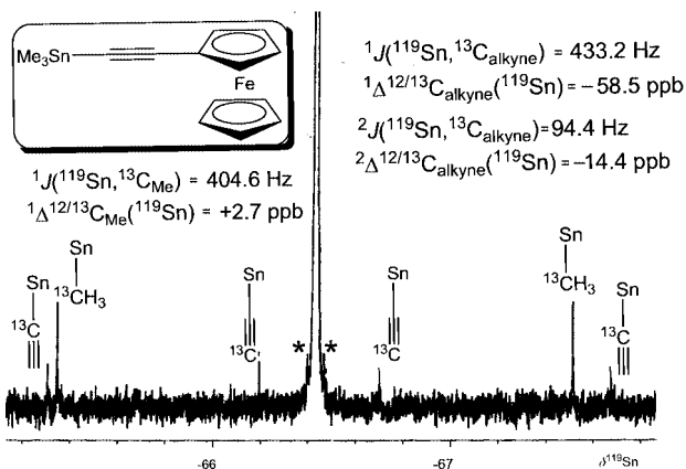
Figure 2. ^{119}\text{Sn}\{^1\text{H}\} NMR spectrum (refocused INEPT [25] ; 186.5 MHz) of ferrocenylethynyl(trimethyl)tin ( 1 ; 5% in \text{CDCl}_3 at 296 K; acquisition time 5 s, repetition delay 2.5 s; 64 transients). The ^{13}\text{C} satellites are marked, and coupling constants and isotope-induced chemical shifts \Delta^{12/13}\text{C}(^{119}\text{Sn}) are given. The ^{13}\text{C} satellites indicated by asterisks correspond to ^3J_{^{119}\text{Sn},^{13}\text{C}_{\text{Fc}}} = 12.8 Hz.
