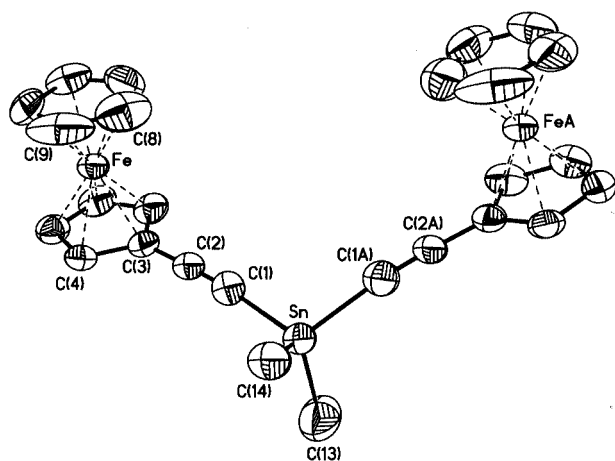
Figure 3. ORTEP representation (50% probability; hydrogen atoms have been omitted) of the molecular structure of bis(ferrocenylethynyl)dimethyltin ( 2 ). Selected bond lengths [pm] and angles [°]: Sn–C1 211.3(8), Sn–C13 211.3(12), Sn–C14 210.0 (12), C1–C2 119.0(9), C2–C3 141.3(9), C3–C4 143.0(8)m, C3–C7 142.2(9), C4–C5 146.1(8), C5–C6 149.2(9), Fe–centroid(C 5 H 4 ) 165.6, Fe–centroid(C 5 H 5 ) 164.4; C1–Sn–C1A 107.0(4), C1–Sn–C13 108.5(3), C1–Sn–C14 109.2(3), C13–Sn–C14 114.3(5), Sn–C1–C2 174.0(6), C1–C2–C3 177.1(7), centroid–Fe–centroid 178.7.
