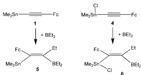
Scheme 3. 1,1-Ethylboration of the (ferrocenylethynyl)tin compounds 1 and 4 .
